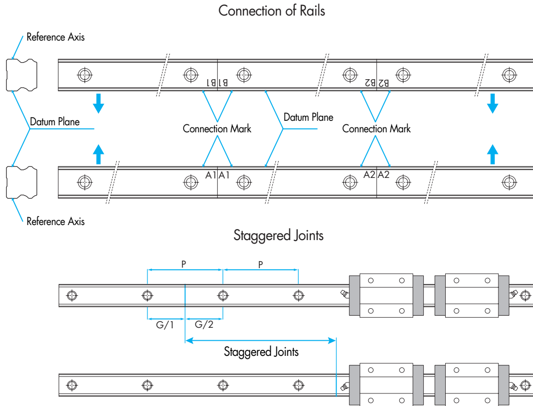
Figure 6. Joining Rails
