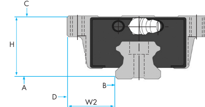
Figure 3. Block measurement
