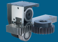
MHD Heavy Duty Track Roller Guidance System
